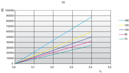
Load / Elongation [ % ]
