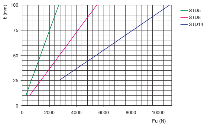
STD profile
